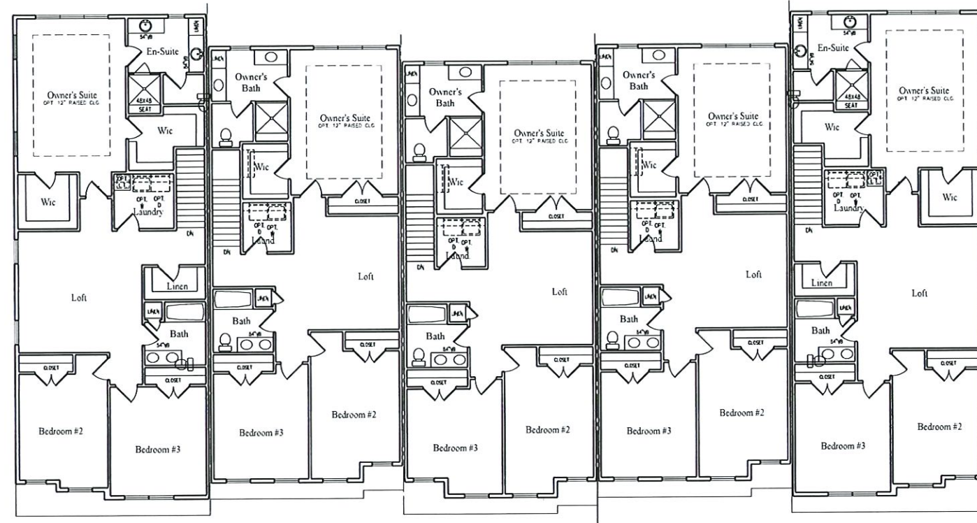
SECOND FLOOR
