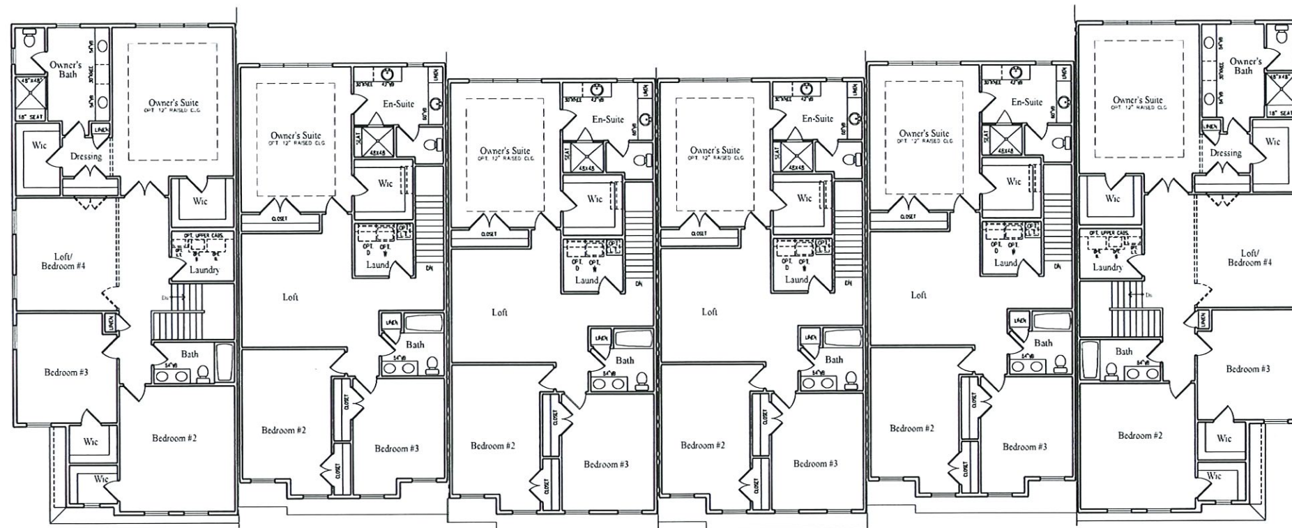
SECOND FLOOR
