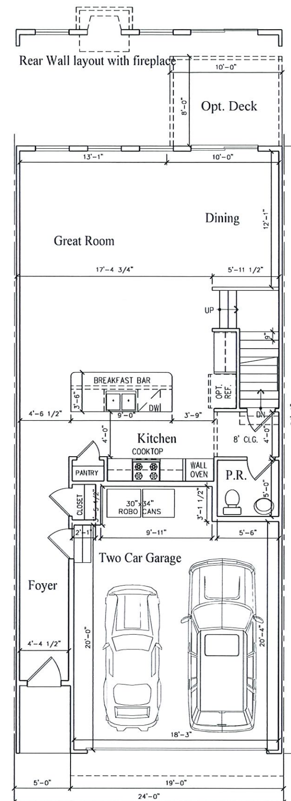
FIRST FLOOR- 848 SQ. FT. GARAGE + STORAGE- 418 SQ. FT. TOTAL: 2,077 SQ. FT.
