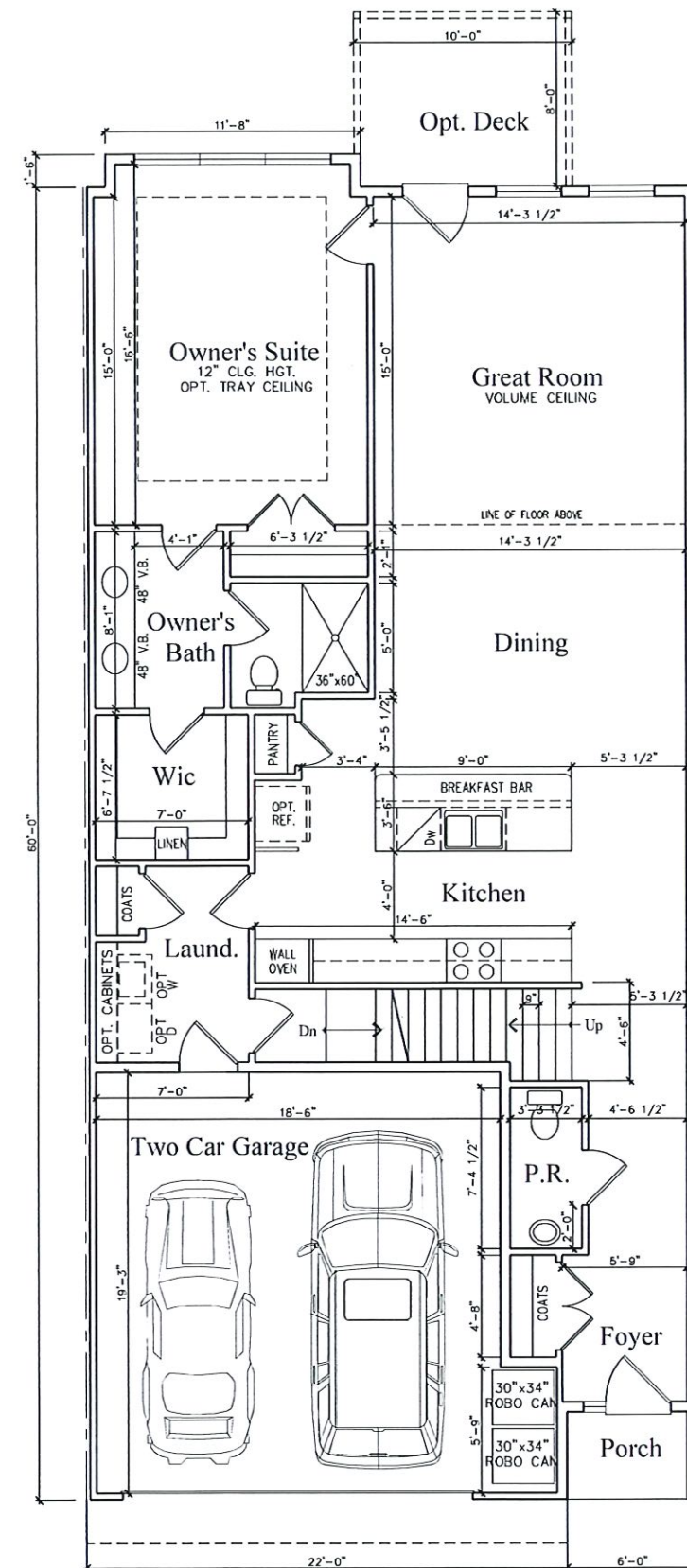
INTERIOR UNIT FIRST FLOOR- 1,286 SQ. FT. GARAGE + STORAGE- 389 SQ. FT. INTERIOR UNIT TOTAL- 2,325 SQ. FT.
