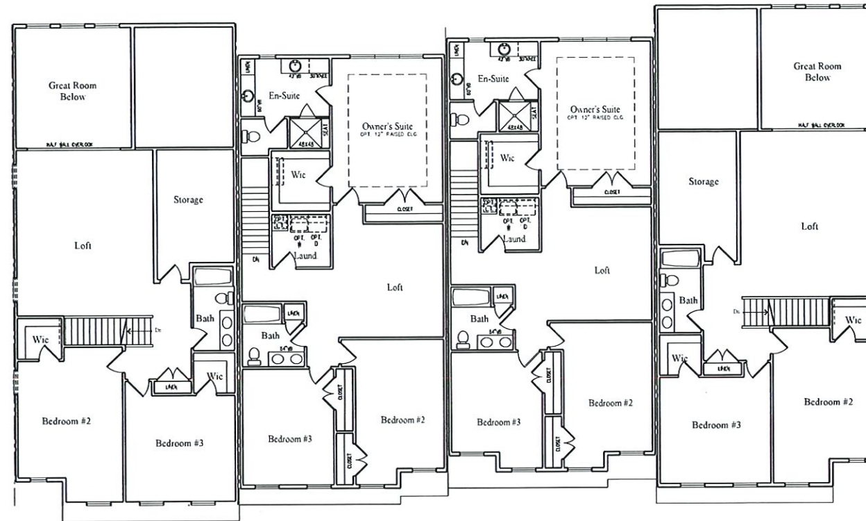
SECOND FLOOR
