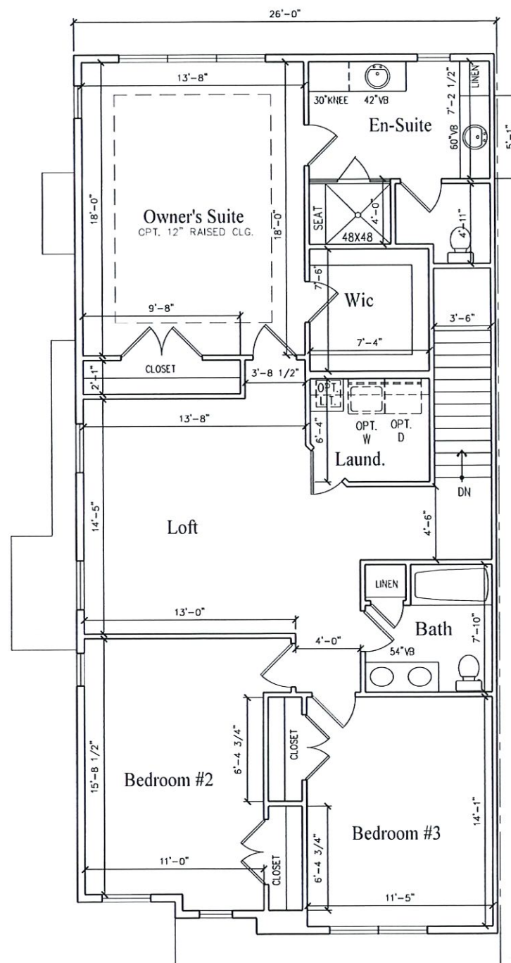
SECOND FLOOR- 1,336 SQ. FT.
