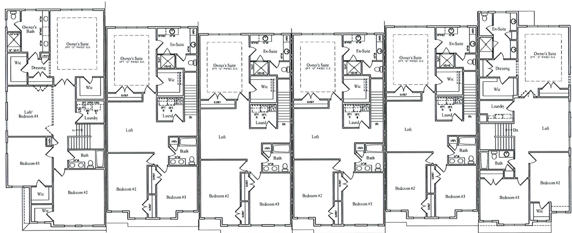
SECOND FLOOR
