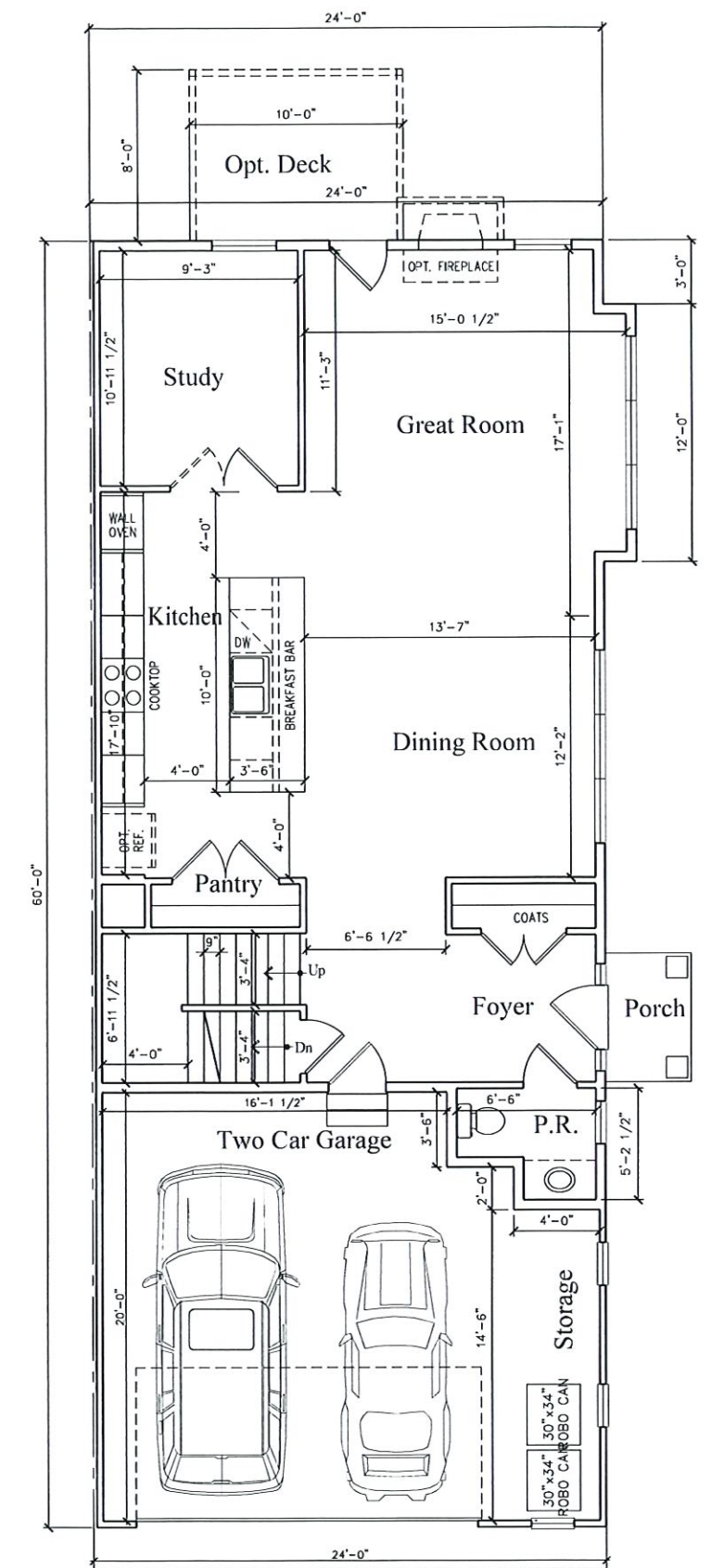
FIRST FLOOR- 1,006 SQ. FT. GARAGE + STORAGE- 452 SQ. FT. TOTAL: 2,365 SQ. FT.
