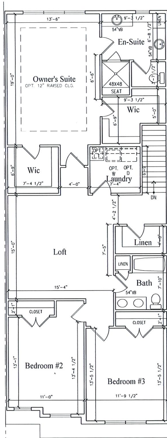
INTERIOR UNIT SECOND FLOOR- 1,386 SQ. FT.
