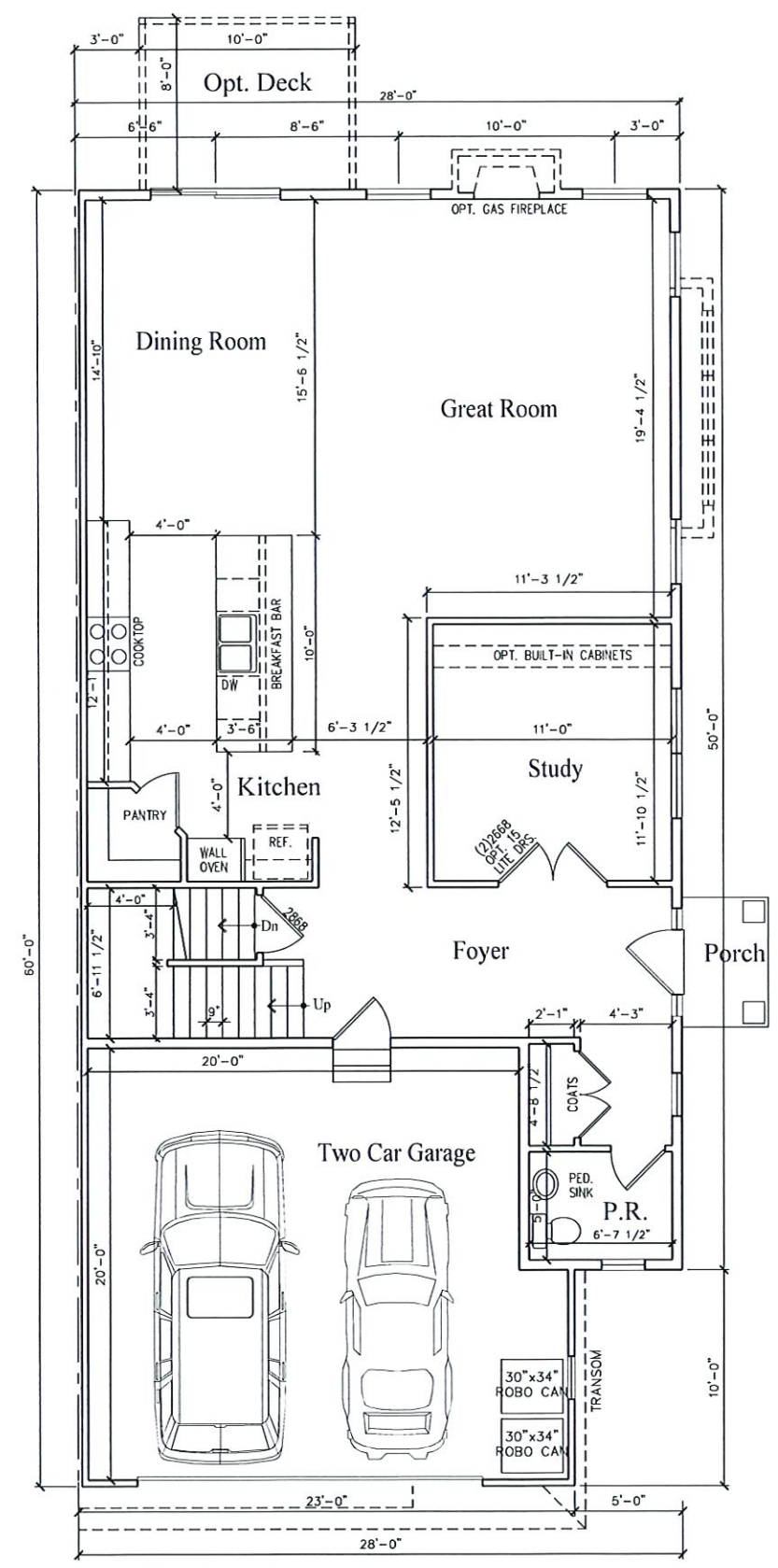
FIRST FLOOR 1,190 SQ. FT. GARAGE + STORAGE 440 SQ. FT. TOTAL: 2,756 SQ. FT.
