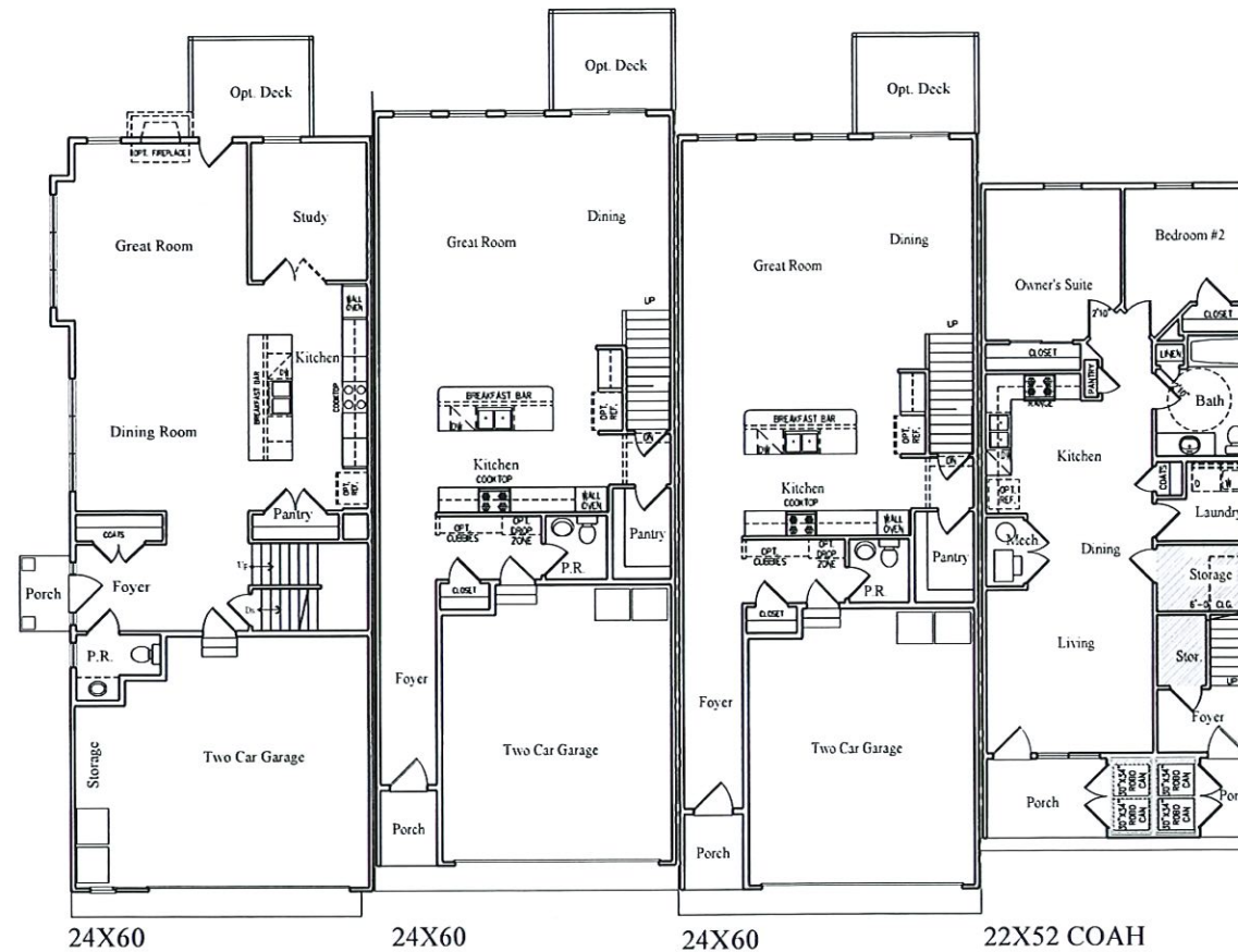
FIRST FLOOR
