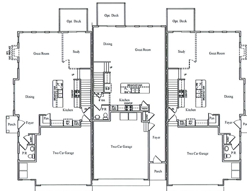
26X54 FIRST FLOOR
