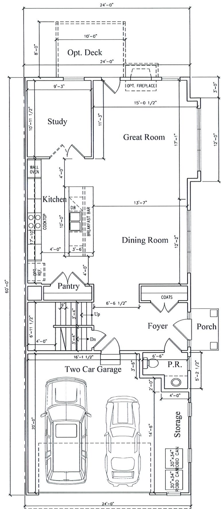
FIRST FLOOR- 1,006 SQ. FT. GARAGE + STORAGE- 452 SQ. FT. TOTAL: 2,365 SQ. FT.
