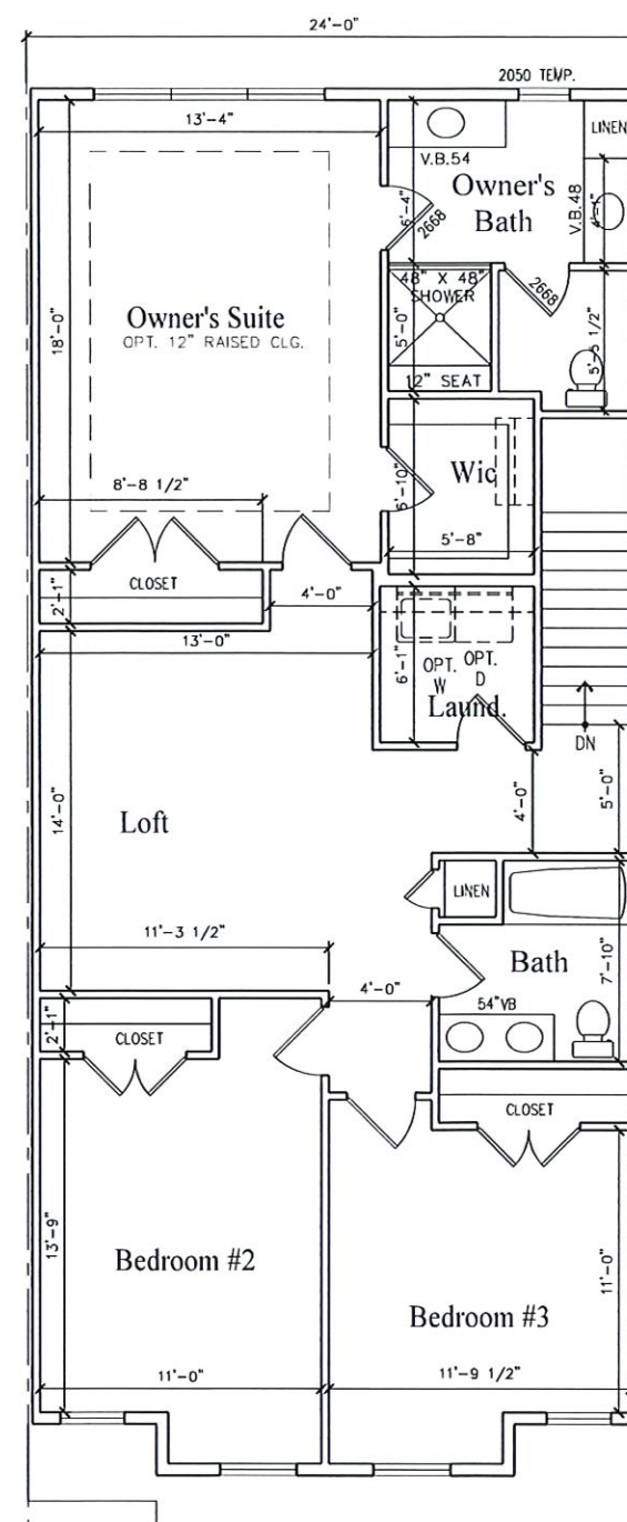
SECOND FLOOR- 1,229 SQ. FT.
