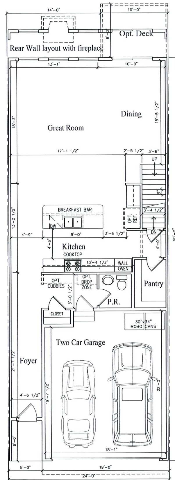
FIRST FLOOR- 1,004 SQ. FT. GARAGE + STORAGE- 406 SQ. FT. TOTAL: 2,390 SQ. FT.
