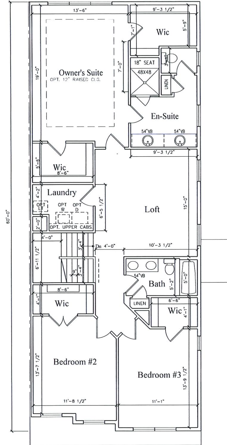
SECOND FLOOR- 1,359 SQ. FT.
