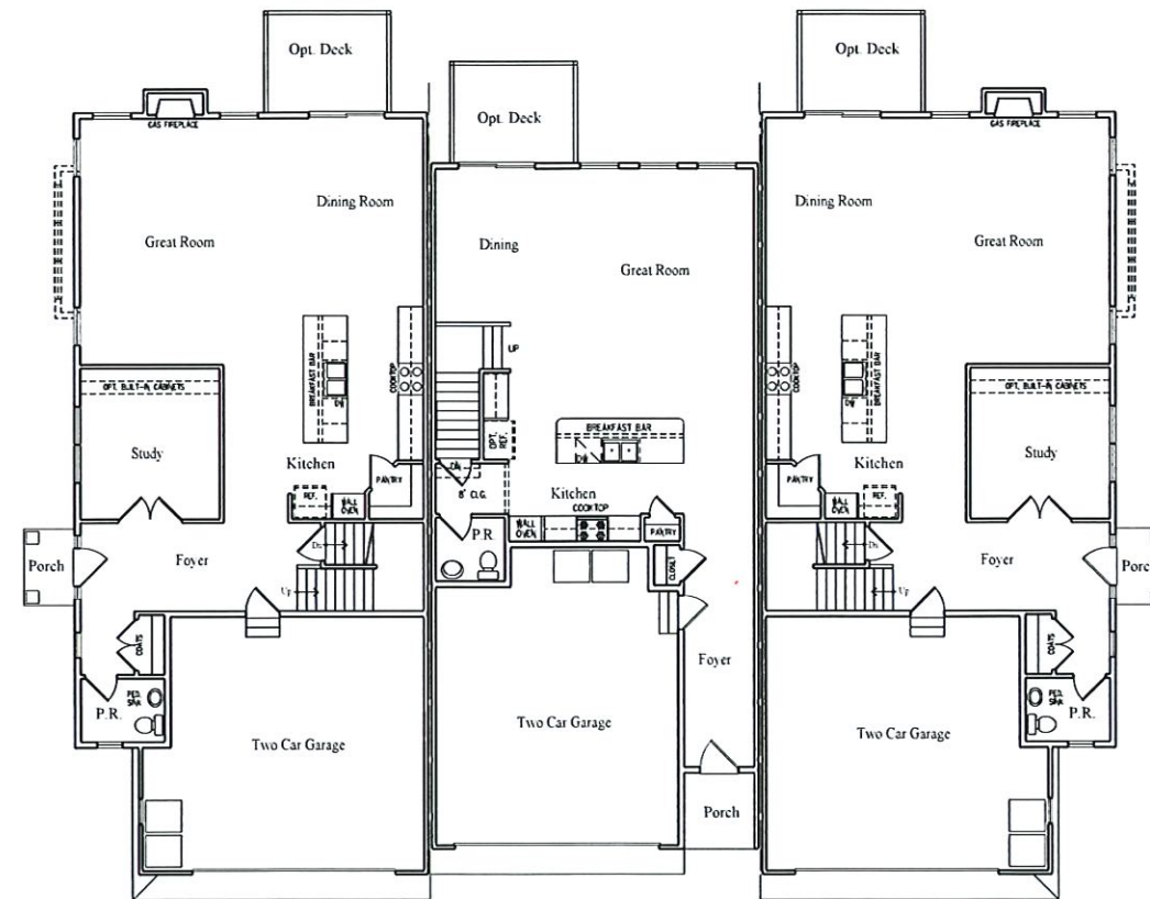
28X60 FIRST FLOOR
